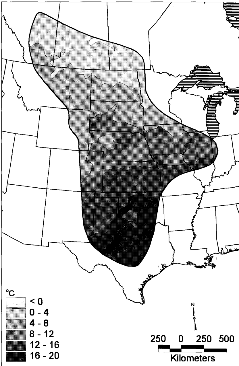
Figure 4. Spatial distribution of mean annual temperature ( ^{\circ}\text{C} ) in the central grassland region of North America (data from Leemans and Cramer 1991).
